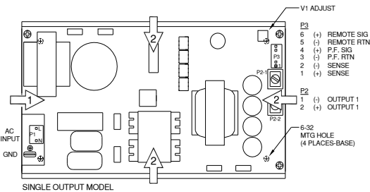
STANDARD CHASSIS
